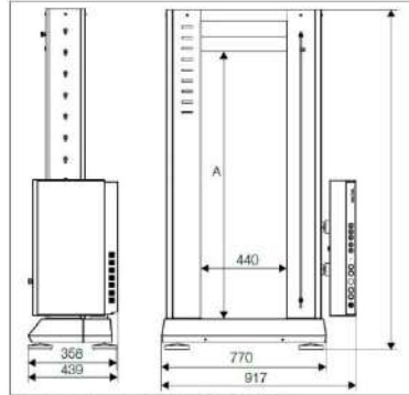
Principle drawing of the ProLine Z005/Z020 TN
